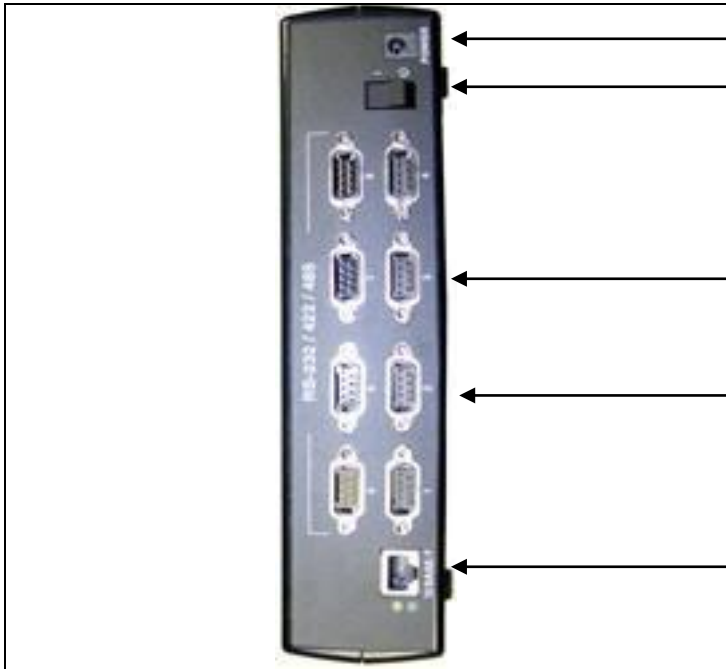
Power connection Power On/OFF switch Female, 9 pin serial connections Female, 9 pin serial connections Ethernet connection
